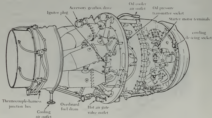
FIGURE 1-34. Accessory location on a centrifugal-flow engine.
